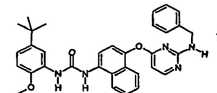
1-[4-(2-Benzylamino-pyrimidin-4-yloxy)-naphthalen-1-yl]-3-(5-tert-butyl-2-methoxy-phenyl)-urea;
